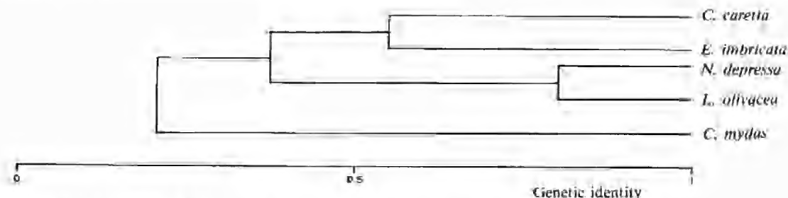
Fig. 1. Dendrogram of chelonid turtle relationships based on electrophoretic data (Table 3).
